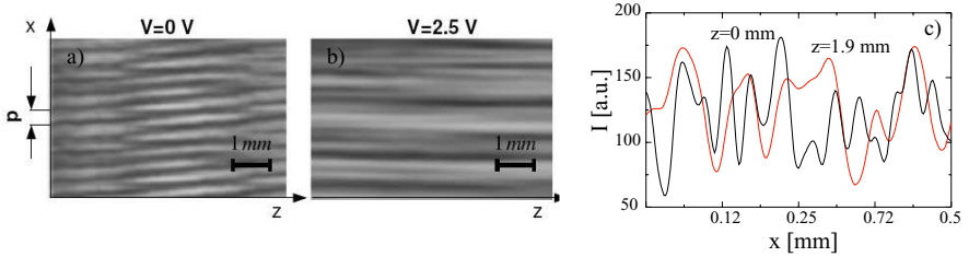
Fig. 4.6 Intensity distribution I(x, z) showing the beam evolution during propagation; a) linear case, b) weakly nonlinear case. c) Two intensity profiles I(x) recorded at z = 0 and z = 1.9 mm in the weakly nonlinear regime, V = 2.5 V.
