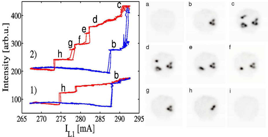
Fig. 9.4 Left panel: Local intensity output emitted by the system when I_{L1} is ramped up and down, for two values of I_{L2} : 1) I_{L2} = 20\text{ mA} , 2) I_{L2} = 22\text{ mA} . The monitored region of the transverse section of the system has a diameter of 80\text{ }\mu\text{m} . Right panel: For each branch indicated by a letter in the left panel we show the corresponding near-field emission profile of the monitored region.
