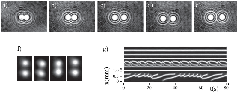
Fig. 5.3 Upper panels: bound states of localized structures obtained for V_0 = 4.5 \text{ V} , I_{in} = 0.5 \text{ mW/cm}^2 and q_b = 3.6 ; all states a)-e) are obtained by inducing a pair of localized structures with an increasing initial distance between centers, and letting the system evolve up to the formation of a stationary bound state. Lower panels: bouncing dynamics of localized structures observed at V_0 = 12.2 \text{ V} and I_{in} = 0.95 \text{ mW/cm}^2 ; f) successive snapshot showing two localized structures bouncing one over the other; g) space-time diagrams showing two stationary localized structures (top), two localized structures with periodic oscillations of their positions (middle) and aperiodic bouncing (bottom).
