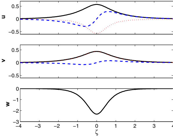
Fig. 3.2 Supersonic gap-acoustic soliton. The solitons's frequency is in the middle of the band gap (soliton parameter Q = \pi/2 ), and it's velocity is \beta_s = 0.25 , which is 125% of the speed of sound, \beta_s = 0.2 . The self- and cross-phase modulation coefficients are \chi_s = 1 , \chi_x = 2 , and the electrostrictive coefficients are \chi_{es} = 1 , \lambda = 0.1 . The first part of the figure shows the amplitude of the envelope u of the forward-moving electromagnetic wave, the second the envelope v of the backward-moving wave, and the third part the acoustic field (material density). Solid lines are for the magnitudes of the amplitudes, dashed lines for the real parts, and dotted lines are for the imaginary parts.
