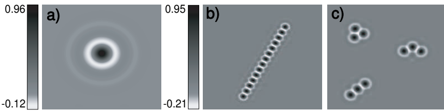
Fig. 7.3 Density plot of the order parameter from a direct numerical simulation of model (7.1), for v = 1 , q = 0.7 and: (a) \varepsilon = -0.088 ; (b) \varepsilon = -0.095 ; (c) \varepsilon = -0.11 .
