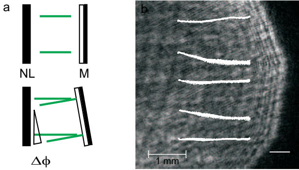
Fig. 11.17 (a)Top: Translational invariant single feedback scheme with a nonlinear optical medium (NL); (Bottom): A small misalignment of the feedback mirror (M) results in a global phase shift \Delta\Phi causing a drift motion; (b): Trajectories of drifting feedback solitons. The trajectories are a superposition of 50 drifting solitons ignited at each of the five addressing positions. Inhomogeneities cause deviations from a straight vertical track and fix the route of the solitons to a trapping route.
