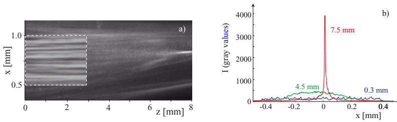
Fig. 4.7 a) Experimental results for intensity distribution I(x, z) for the same parameter values for Fig.4.6. Area marked by the dashed line is shown at a higher resolution (using a larger magnification objective). b) Linear intensity profiles I(x) taken at different propagation distances, z = 0.3, 4.5 and 7.5 mm
