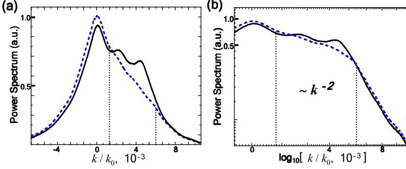
Fig. 2.9 Detailed look at the asymptotic spectral profile of the turbulent state during multiple BOT instability. (a) Comparison of input (solid) and output (dashed) profiles. (b) Comparison in log space, showing algebraic spectrum in interaction region.
