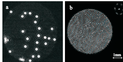
Fig. 11.4 Example of spatial structures in the polarization mode; a: solitary structures at \psi_1 = -\psi_1 = 44^\circ , V_{ext} = 4.3 V, and propagation length L = -20 cm; b: a hexagonal pattern at U_{ext} = 4.7 V. The far field is shown in the upper right corner.
