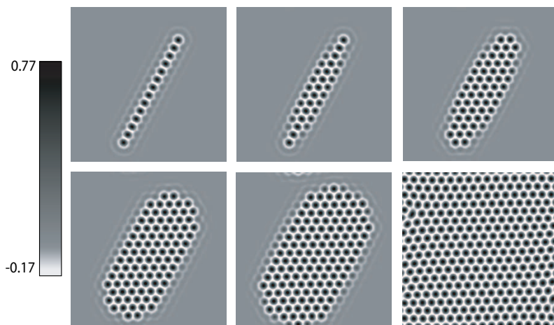
Fig. 7.6 Density plot of the order parameter from a direct numerical simulation of model (7.1) for v = 0.9 , q = 0.7 and \varepsilon = -0.075 . Time runs from left to right and from top to bottom.
