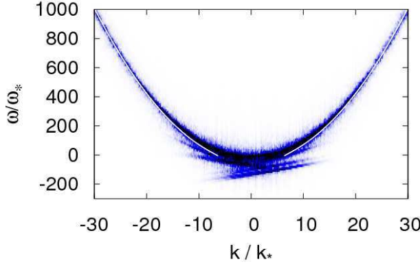
Fig. 4.9 The k - \omega spectrum of the wave field at z = 2.1 \text{ m} . \omega_* = 1/256ql_\xi^2 and k_* = 1/\sqrt{128}l_\xi . The Bogoliubov dispersion relation is shown by the solid line.
