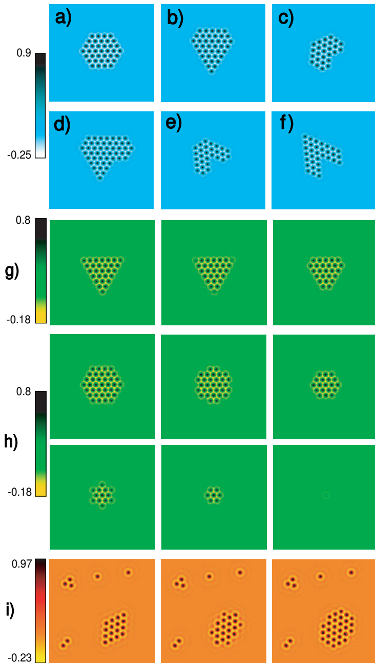
Fig. 7.2 Density plot of the order parameter from a direct numerical simulation of model (7.1), for \nu = 1 , q = 0.7 and: (a) \varepsilon = -0.12 ; (b) \varepsilon = -0.12 ; (c) \varepsilon = -0.12 ; (d) \varepsilon = -0.135 ; (e) \varepsilon = -0.14 ; (f) \varepsilon = -0.135 ; (g) \varepsilon = -0.151 (temporal evolution, time runs from left to right); (h) \varepsilon = -0.155 (temporal evolution, time runs from left to right and from top to bottom); (i) \varepsilon = -0.09 (temporal evolution, time runs from left to right).
