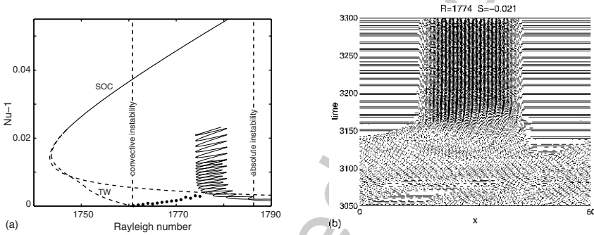
Fig. 6.1 (a) Bifurcation diagram showing the time-averaged convective heat flux per unit length across the layer, Nu-1 \equiv \Gamma^{-1} \int_{-\Gamma/2}^{\Gamma/2} \theta_z(x, z=1) dx , as a function of the Rayleigh number R when \Gamma = 60 . The conduction state loses instability at a Hopf bifurcation ( R = R_H \approx 1760.8 ). Steady spatially periodic convection (SOC) acquires stability at a parity breaking bifurcation marking the destruction of a branch of spatially periodic traveling waves (TW) originating in the primary bifurcation. Small amplitude dispersive chaos (solid dots) is present for R > R_H and leads into the pinning region ( 1774 < R < 1781 ) containing a multiplicity of stable localized states of both even and odd parity. (b) Space-time plot showing the midplane temperature \theta(x, z = 1/2, t) as a function of time for R = 1774 starting from a random small amplitude initial condition. Parameters: S = -0.021 , \sigma = 6.22 , \tau = 0.009 , \Gamma = 60 . From Ref. [9].
