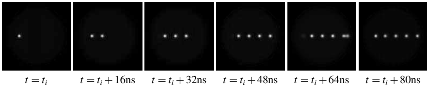
Fig. 8.11 Sequence of snapshots showing the spatio-temporal dynamics of drifting CSs in the transverse section of the VCSEL in presence of a defect. Intensity increases from black to white. The position of the defect corresponds to the high intensity structure visible in the first panel, and the phase gradient is directed rightwards. Defect characteristics: \theta_0 = -2.0472 , \theta_d = 0.25 , \sigma_d = 11.25 \mu\text{m} . Other parameters: E_I = 0.792 , I = 2.0024 , K = 0.052 \mu\text{m}^{-1} , and t_i = 5 \text{ ns} is the time after initiation of the phase gradient in the numerical simulation.
