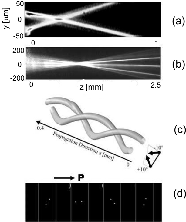
Fig. 1.5 (a) In plane crossing of two identical nematons. (b) Multiple soliton generation by a focused light beam. (c) Out-of-plane attraction between two skew nematons. (d) The photographs taken at the output of the cell show that, as the excitation increases, the cluster rotates faster in propagation, with a power-dependent angular change ( \pi , in this set)
