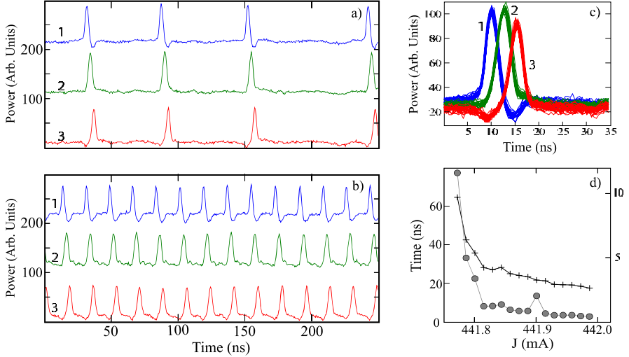
Fig. 8.10 a): Intensity outputs from a linear array of four detectors placed along a channel line and separated by 9\ \mu\text{m} . Detector 1 monitors the defect point where the structure forms, no intensity is monitored by the last detector of the array (detector 4) and its trace is not shown. Each trace is vertically shifted for clarity. The VCSEL current is J = 441.76\text{mA} and holding beam intensity is 15\text{ mW} . b): As in a) except for VCSEL current which is J = 442.0\text{mA} . c): For the case depicted in a), we superimpose fifty spatio-temporal sequences monitored by three detectors. d): Average period of the sequence in a) \langle T \rangle (crosses, with left vertical scale) and its standard deviation \sigma(T) (circles, with right vertical scale) as a function of J .
