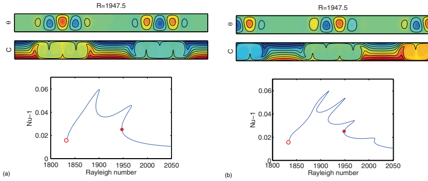
Fig. 6.7 Odd parity multicongvectons with NBC. (a) A bound pair of “even” parity convectons of opposite sign. (b) A bound pair of “odd” parity convectons. Lower panels show the bifurcation diagrams with the red dot indicating the location of the profile shown in the upper panel. The open dots indicate the termination point of each branch; this point is the same for both branches and lies on a branch with 13 identical cells (not shown). Parameters: S = -0.1 , \sigma = 7 , \tau = 0.01 . From Ref. [43].
